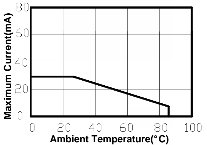
Maximum Current & Ambient Temperature
