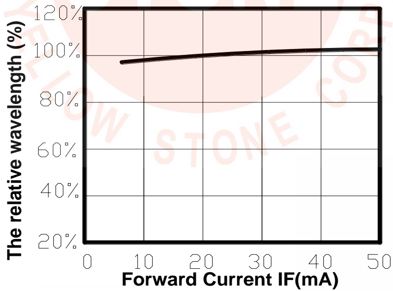
The relative Wavelength & Forward current
