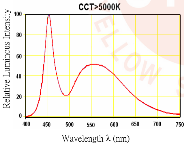
Fig.3 Wavelength Characteristics(Ta=25°C)
