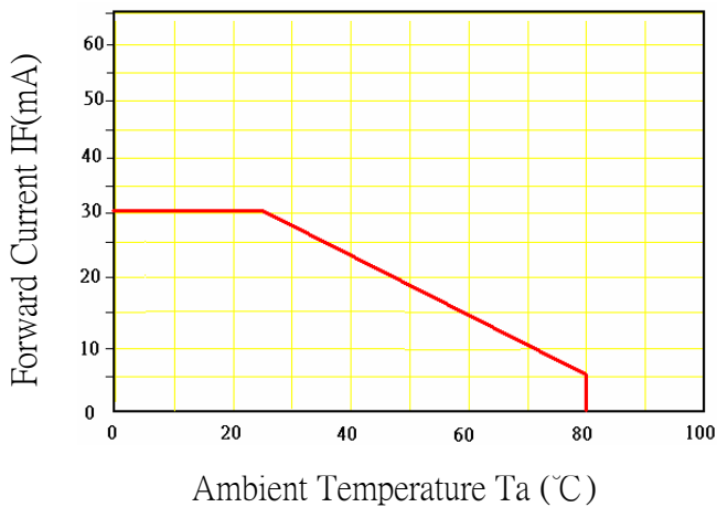
Fig.5 IF-Ta
