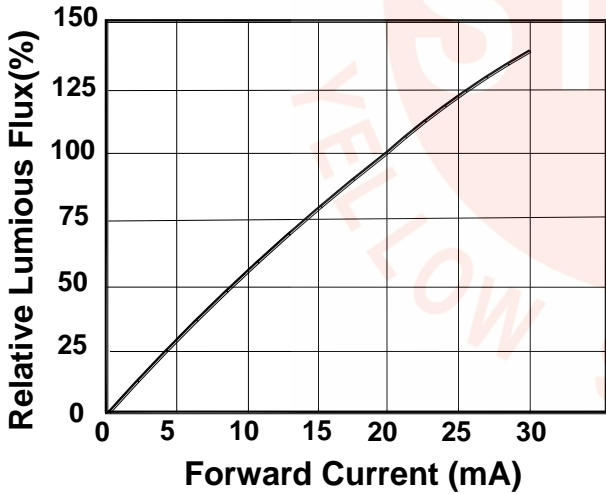
Relative Luminous Flux .Current Ta=25
