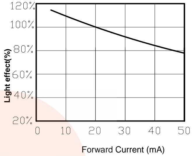
Light effect VS Current
