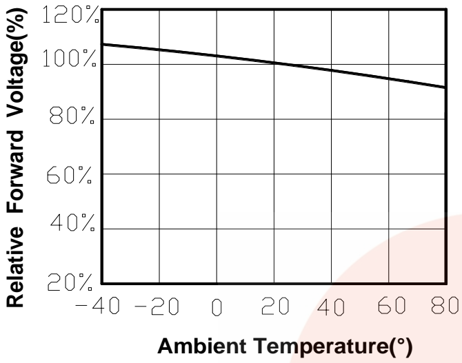
Forward Voltage Temperature
