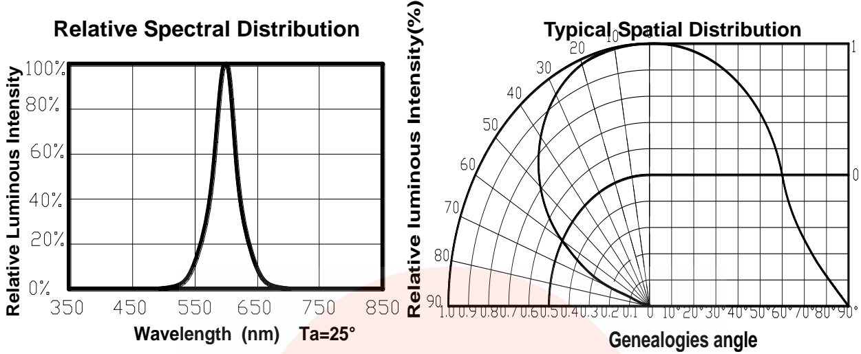
Relative Luminous Flux .Current Ta=25
