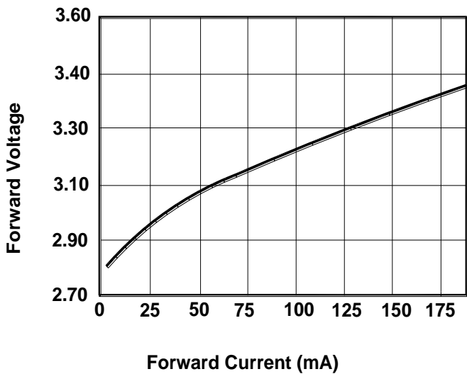
Electrical Characteristics
